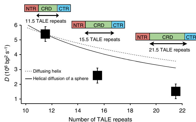
Figure 5 | Effect of CRD size on 1D diffusion coefficient of TALE proteins.
