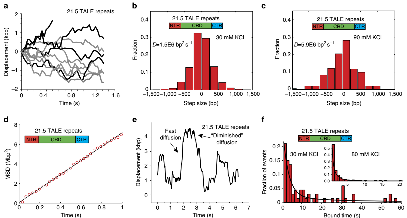
Figure 3 | TALE proteins exhibit rapid 1D diffusion along DNA templates. (a) Single-molecule trajectories of TALE diffusion events over short timescales ( \sim 1 s) at 90 mM KCl. (b,c) Histograms of TALE step sizes along non-specific DNA at 30 and 90 mM KCl, respectively. The number of trajectories, n , is 50 for both conditions. (d) Mean-squared displacement of an ensemble of TALE proteins diffusing along non-specific DNA templates at 90 mM KCl. The values are averages of n = 50 trajectories. (e) Single-molecule trajectory at 90 mM KCl over long timescales ( > 5 s) shows periods of rapid diffusion interspersed with periods of diminished diffusion. (f) Distribution of characteristic TALE bound times at 30 mM KCl and (inset) 80 mM KCl with corresponding double-exponential fits. The number of events recorded, n , is equal to 70 and 250 for 30 and 80 mM KCl, respectively.
