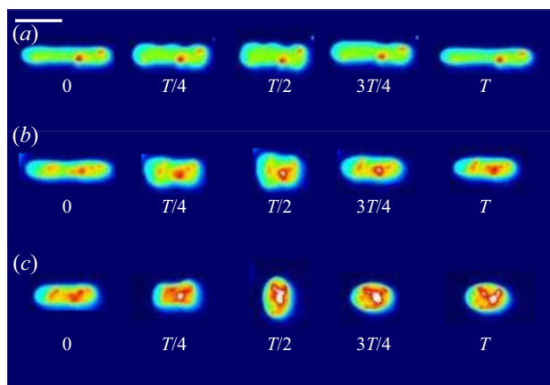
Figure 12. Dynamics of a tubular vesicle with reduced volume \nu = 0.64 \pm 0.02 in LAOE. (a) Snapshots showing pulsating dynamics of a vesicle over one sinusoidal strain rate input cycle with time period T = 4 s at Ca = 21.3 and De = 17.7 . (b) Snapshots showing pulsating dynamics with wrinkles of a vesicle over one sinusoidal strain rate input cycle with time period T = 8 s at Ca = 21.3 and De = 8.9 . (c) Snapshots showing change in the 2-D shape of a vesicle over one flow cycle with time period T = 15 s at Ca = 21.3 and De = 4.7 . Scale bar is 20 \mu\text{m} . False colouring is applied to the greyscale images for resolution enhancement.
