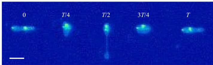
Figure 14. Asymmetric dumbbell formation in a vesicle with reduced volume \nu = 0.69 exposed to LAOE flow at Ca = 52.5 and De = 1.2 . Scale bar is 10\ \mu\text{m} .
