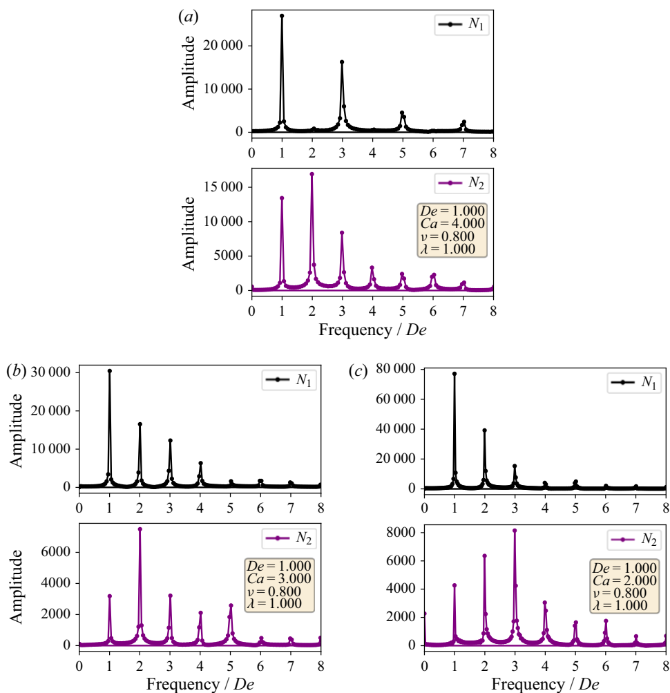
Figure 11. Fourier decompositions of the stress responses for indicative parameter sets in each of the dynamical regimes. The panels are (a) symmetrical regime; (b) reorienting regime; (c) pulsating regime.
