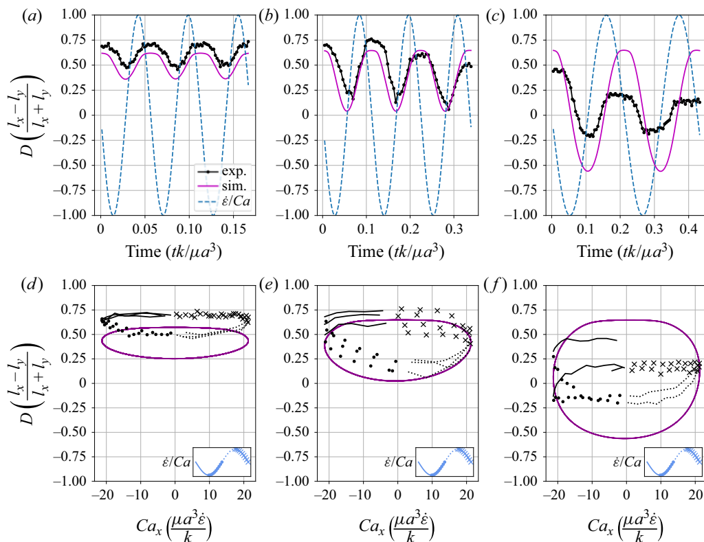
Figure 13. Experimental and simulation single vesicle Lissajous curves and deformation plots for \nu = 0.64 . For each panel: (a) Ca = 21.3 , De = 17.7 , \nu = 0.64 ; (b) Ca = 21.3 , De = 8.9 , \nu = 0.64 ; (c) Ca = 21.3 , De = 4.7 , \nu = 0.64 ; (d) Ca = 21.3 , De = 17.7 , \nu = 0.64 ; (e) Ca = 21.3 , De = 8.9 , \nu = 0.64 ; (f) Ca = 21.3 , De = 4.7 , \nu = 0.64 .
