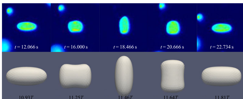
Figure 4. Comparison of the experimental and simulation vesicle shapes in the symmetrical regime over one flow cycle at the same conditions of Ca = 10.9 , De = 3.0 , \nu = 0.88 , \lambda = 1.00 . The times in the figure are in seconds for the experimental movie. Shapes from the simulations at the same non-dimensional cycle times are shown below. Here T is the non-dimensional period, defined as T = 1/De .
