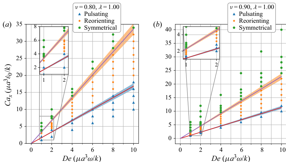
Figure 8. Phase diagrams for the low to medium to high deformation regimes for vesicles of reduced volume \nu = 0.80 and \nu = 0.90 . Lines in the diagrams are from the semianalytical theory presented near the end of § 3.1. Due to uncertainty in determining the D_o value, a 5 % error has been included on the lines.
