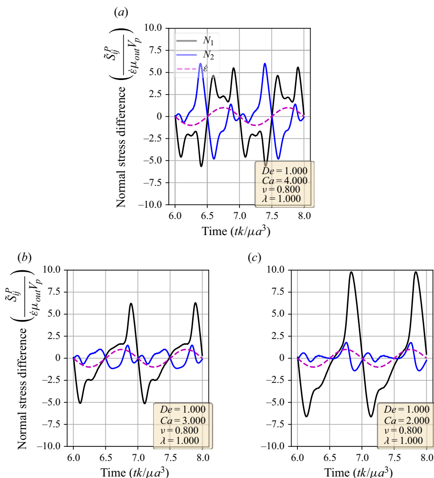
Figure 9. Normal stress differences versus time for simulations in the pulsating, reorienting and symmetrical regimes. Data over two strain rate cycles is plotted. The \dot{\epsilon}/Ca dotted line is the strain rate of the external flow; it is used to show the directionality of the flow. Parameters used are included in the figure legends. The panels are (a) symmetrical regime; (b) reorienting regime; (c) pulsating regime.
