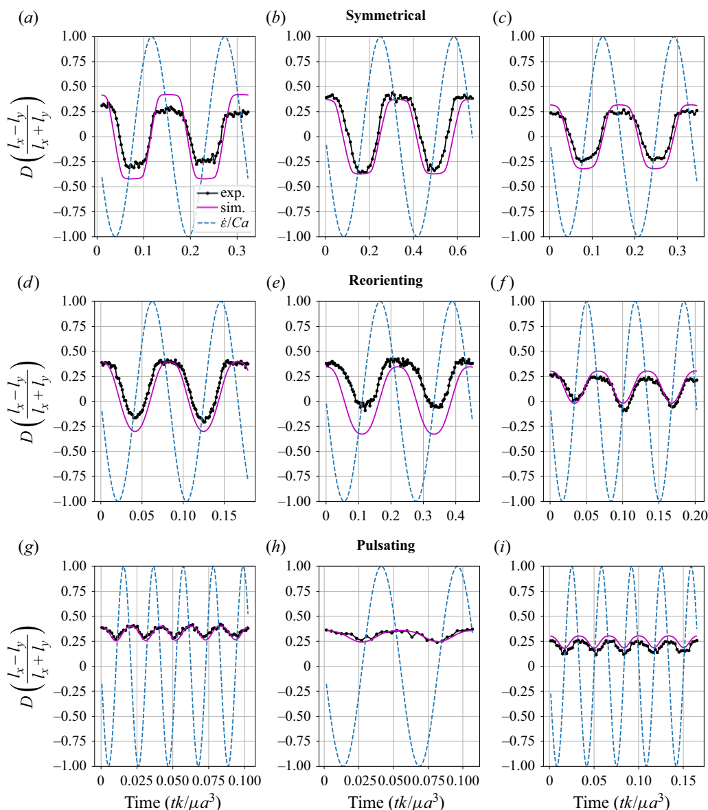
Figure 2. Transient deformation parameter D for vesicle dynamics in time-dependent LAOE from experiments and simulations. All vesicles have a viscosity ratio of \lambda = 1.0 . The \dot{\epsilon}/Ca line is the instantaneous strain rate of the external flow along the x -axis. A negative \dot{\epsilon}/Ca value is compression along the x -axis. For each panel: (a) Ca = 28.8 , De = 6.40 , \nu = 0.85 ; (b) Ca = 10.9 , De = 3 , \nu = 0.88 ; (c) Ca = 17.9 , De = 6 , \nu = 0.91 ; (d) Ca = 28.8 , De = 12 , \nu = 0.85 ; (e) Ca = 10.9 , De = 4.5 , \nu = 0.88 ; (f) Ca = 17.9 , De = 14.9 , \nu = 0.91 ; (g) Ca = 28.8 , De = 48 , \nu = 0.85 ; (h) Ca = 10.9 , De = 18.2 , \nu = 0.88 ; (i) Ca = 17.9 , De = 29.9 , \nu = 0.91 .
