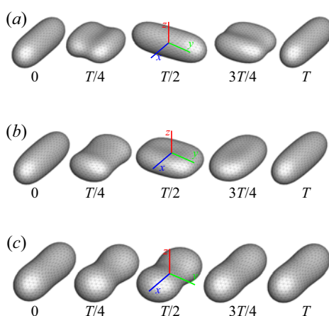
Figure 5. Snapshots of vesicle shapes from simulations over a flow cycle for the three dynamical regimes. The values under the figures are fractions of a strain rate period defined as T = 1/De .
