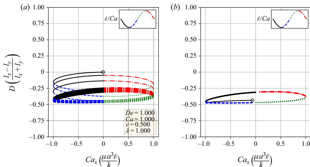
Figure 7. Lissajous-type deformation parameter curves from an oblate shape initial condition and a prolate shape initial condition. The legend at the top right in each panel indicates colour coding for the strain rate cycle. The black circle marks the deformation parameter of the initial shape. The panels are (a) oblate initial; (b) prolate initial.
