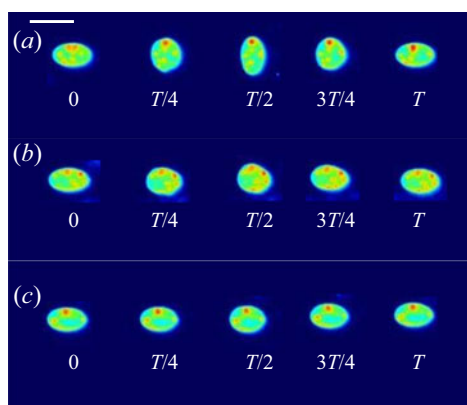
Figure 6. Snapshots of vesicle shapes from experiments over a flow cycle for the three dynamical regimes. The values under the figures are fractions of cycle time T in seconds. Scale bar is 20\ \mu\text{m} . False colour is applied to the greyscale images for enhancing the resolution.
