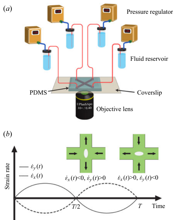
Figure 1. Stokes trap for studying vesicle dynamics in LAOE flow. (a) Schematic of the experimental set-up used to generate planar extensional flow. Inlet/outlet channels in the polydimethylsiloxane (PDMS) microfluidic device are connected to fluidic reservoirs containing the vesicle suspension and pressurized by regulators controlled by a custom LabVIEW program, thereby generating pressure-driven flow in the cross-slot. (b) Schematic of the sinusoidal strain rate input function for one full cycle. The insets are schematics showing the oscillatory extensional flow profile in the microfluidic cross-slot device during the first half ( 0 < t < T/2 ) and second half-period ( T/2 < t < T ) of the cycle.
