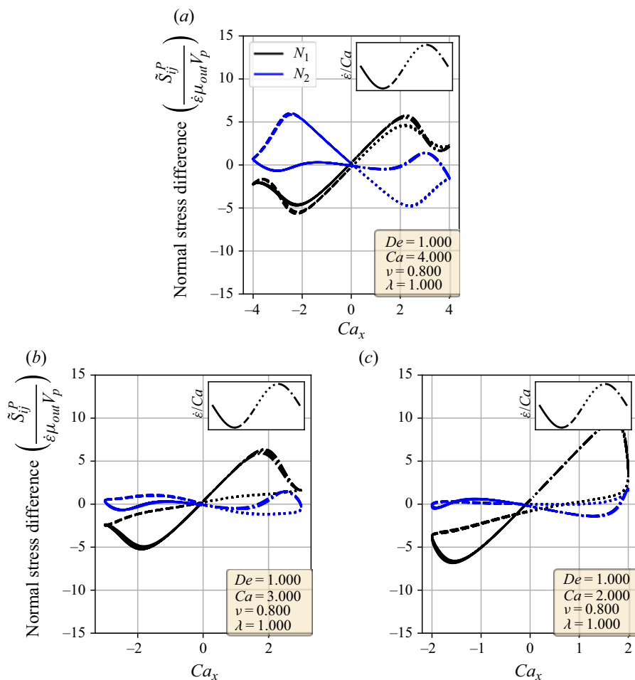
Figure 10. Lissajous-type normal stress difference versus strain rate ( Ca_x ) curves for simulations in the pulsating, reorienting and symmetrical regimes. The strain rate cycle is separated into four periods demarcated by the line formatting. Parameters used are included in the figure legends. The panels are (a) symmetrical regime; (b) reorienting regime. (c) pulsating regime.
