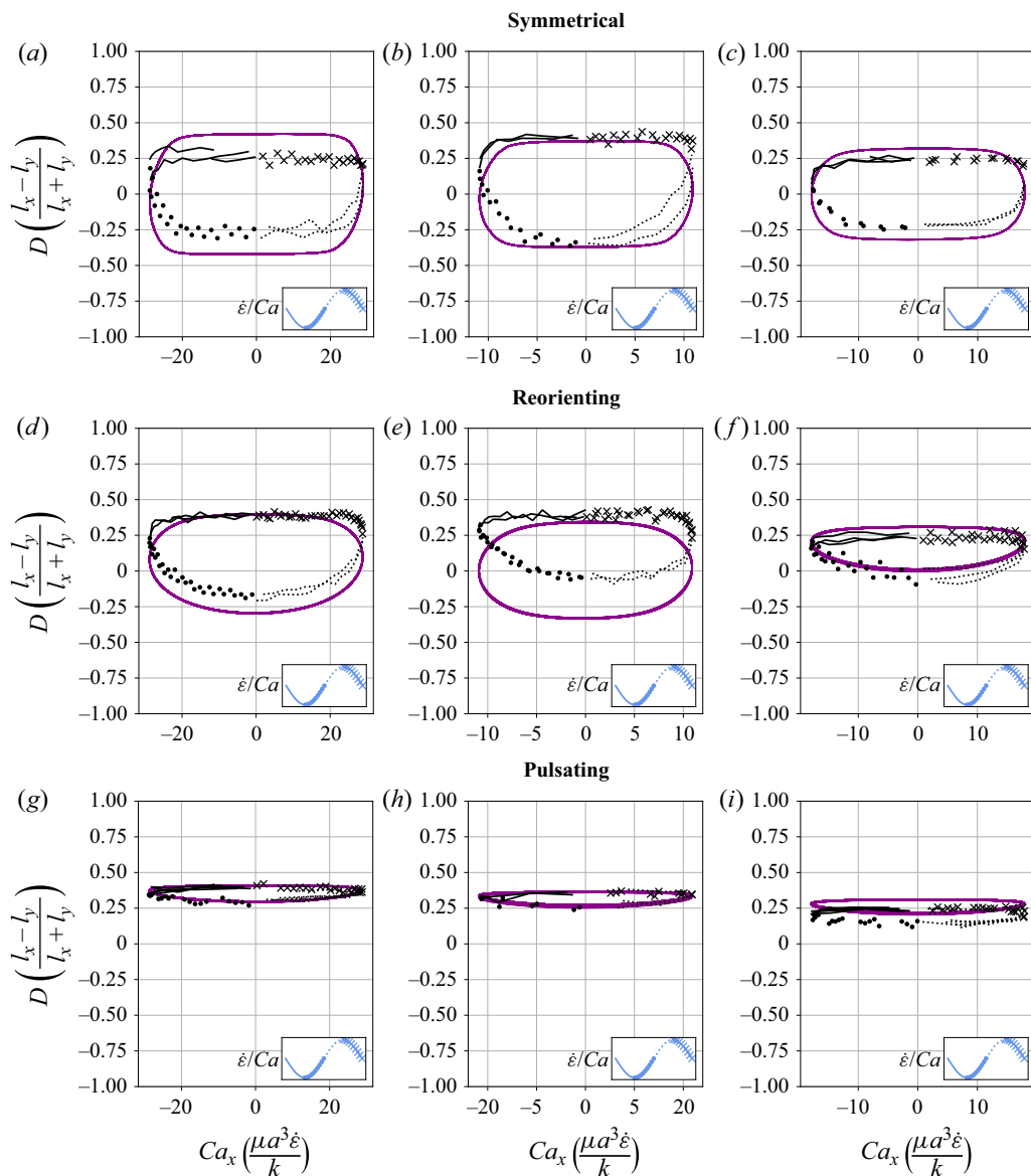
Figure 3. Lissajous-type curves of the deformation parameter D versus the dimensionless instantaneous strain rate. All vesicles have a viscosity ratio of \lambda = 1.0 . Black data points are experimental data; purple data points show numerical data. The oscillatory strain rate cycle is separated into four parts that have been noted with different markers, as shown in the legend in the bottom right-hand corner of each panel. For each panel: (a) Ca = 28.8 , De = 6.4 , \nu = 0.85 ; (b) Ca = 10.9 , De = 3 , \nu = 0.88 ; (c) Ca = 17.9 , De = 6 , \nu = 0.91 ; (d) Ca = 28.8 , De = 12 , \nu = 0.85 ; (e) Ca = 10.9 , De = 4.5 , \nu = 0.88 ; (f) Ca = 17.9 , De = 14.9 , \nu = 0.91 ; (g) Ca = 28.8 , De = 48 , \nu = 0.85 ; (h) Ca = 10.9 , De = 18.2 , \nu = 0.88 ; (i) Ca = 17.9 , De = 29.9 , \nu = 0.91 .
